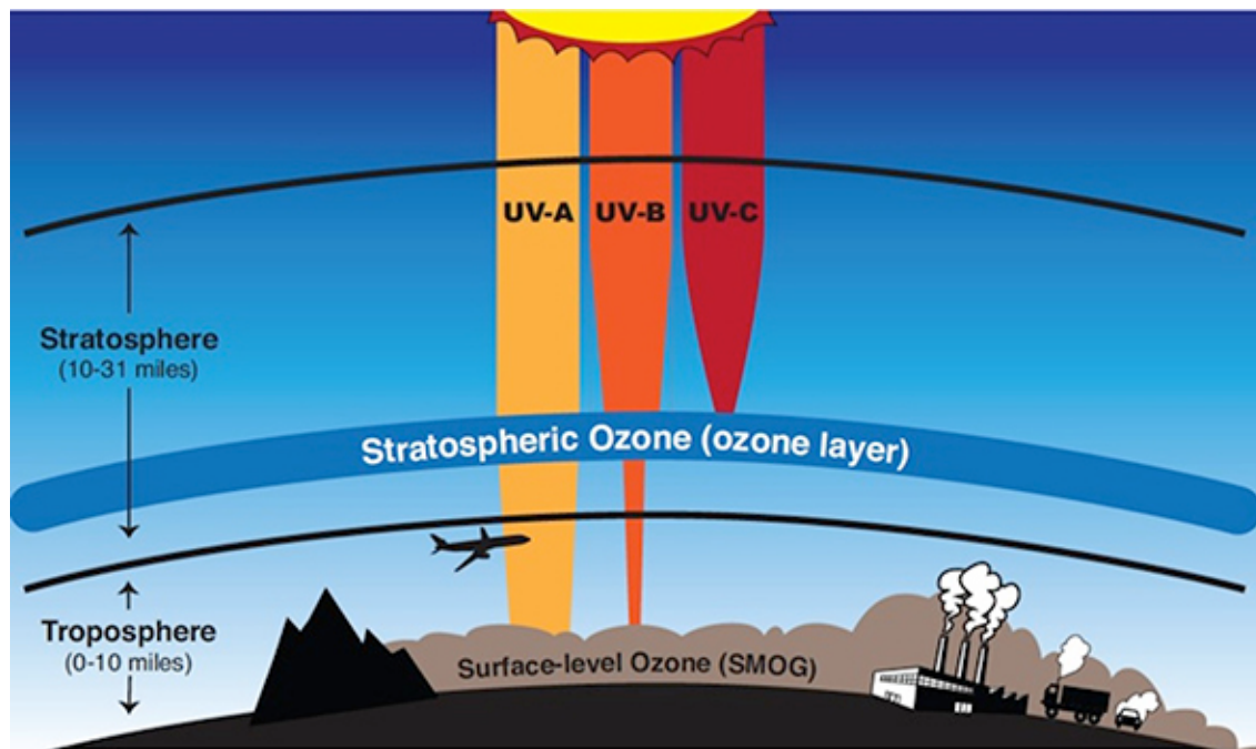
Figure 5. The ozone layer absorbs UV-B and UV-C light, protecting life on Earth from its harmful effects. This Photo by NASA is licensed under CCO Public Domain.
