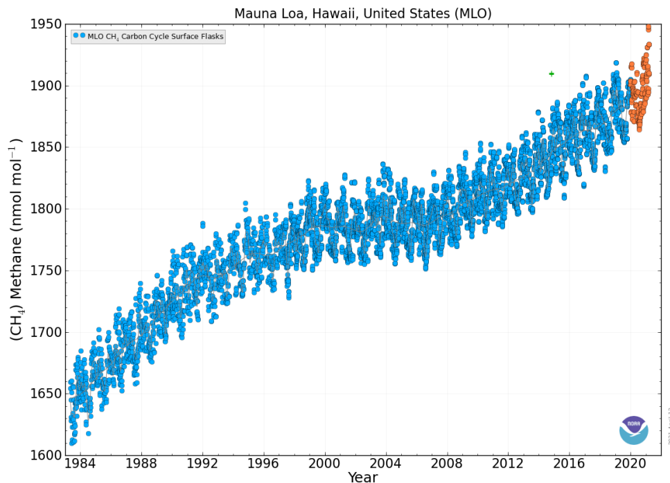
Figure 10: Top: Atmospheric methane concentrations as a function of time. Top: Recent air measurements from Mauna Loa. Bottom: Ice core, firn, and air measurements from Antarctica. Note that most methane sources are in the northern hemisphere, which leads to higher concentrations there compared with the southern hemisphere.
