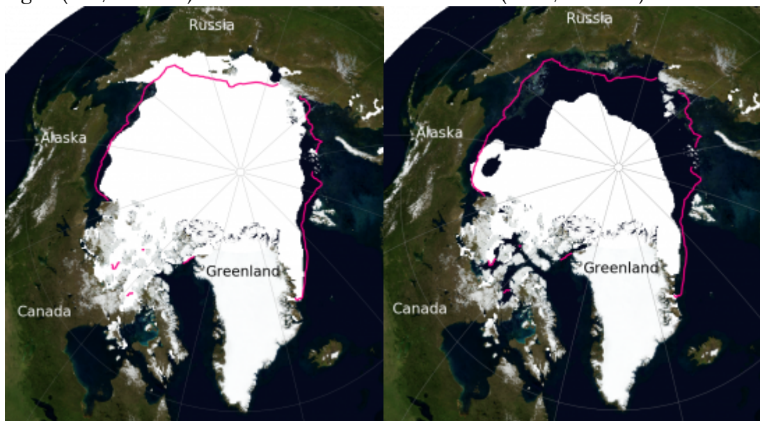
Figure 3: Arctic sea ice extent in September 1979 (left) and 2020 (right) from satellite observations. The purple line denotes the median ice extent from 1981-2010. In 1979 the ice extent was 7.1 million
