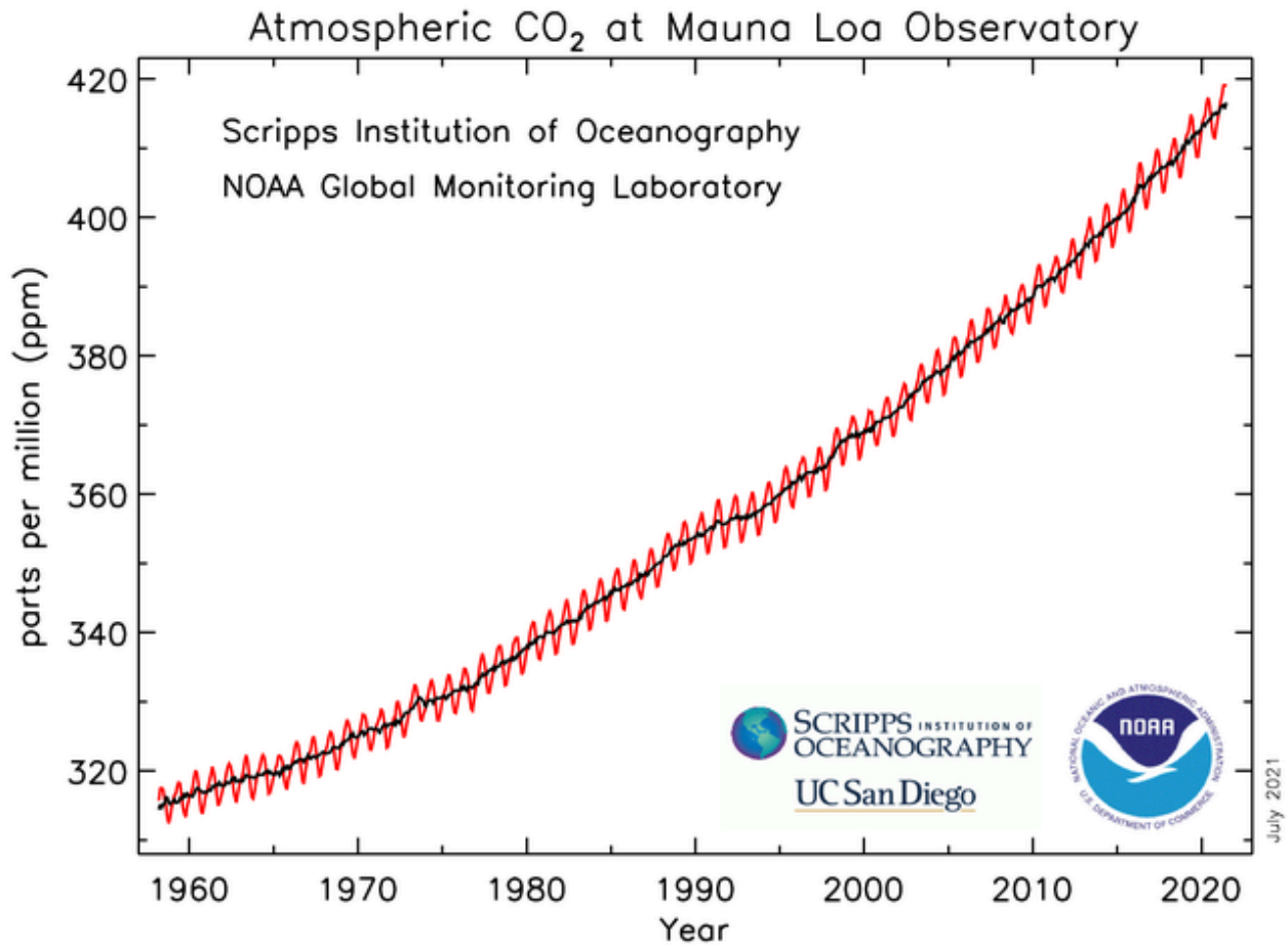
Figure 10: Atmospheric CO 2 measured at Hawaii’s Mauna Loa Observatory. The measurements were pioneered by Charles Keeling from Scripps Institution of Oceanography in 1958. From noaa.gov .
