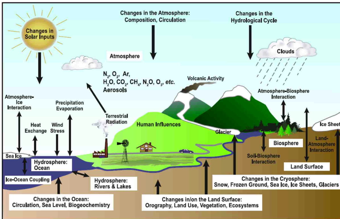
Figure 2: Schematic view of components of the climate system and processes involved in their interactions. From Le https://www.ncdc.noaa.gov/cagTreat et al. (2007).
