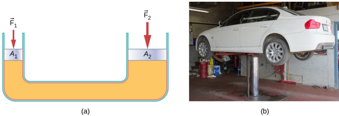
Figure 14.17 (a) A hydraulic jack operates by applying forces ( F_1, F_2 ) to an incompressible fluid in a U-tube, using a movable piston ( A_1, A_2 ) on each side of the tube. (b) Hydraulic jacks are commonly used by car mechanics to lift vehicles so that repairs and maintenance can be performed. (credit b: modification of work by Jane Whitney)
